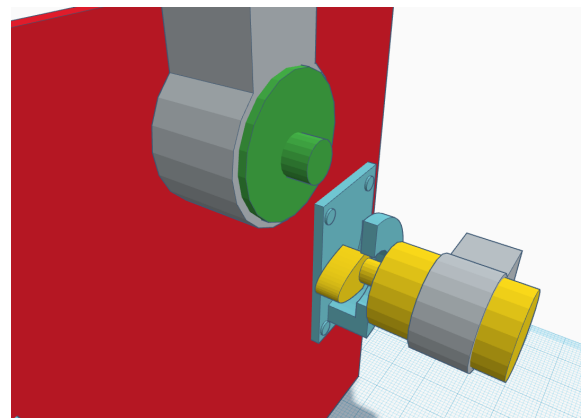
Fig. 9. When the arms are rotated out from the metal plate, the container is unlocked and can manually be opened.
