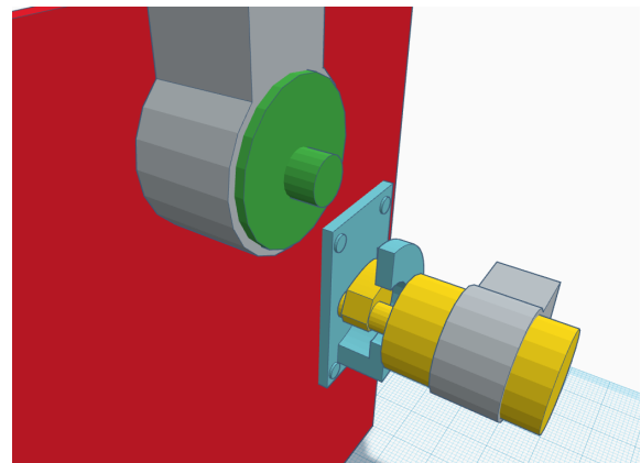
Fig. 8. When the motor arms are under the metal plate, the container remains locked
