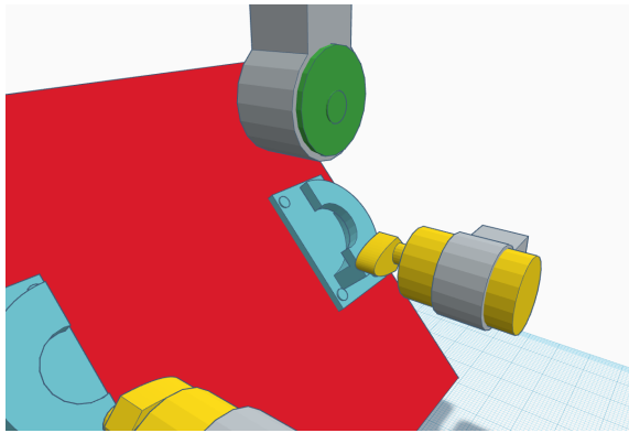
Fig. 10. The internal solenoid can be used for several effects. For example, when facing the container opening, it can pop the door open automatically. If it is facing a wall, it will create a knock sound, or if it does not contact with anything, it can make a clicking noise to signal the box is unlocked.
